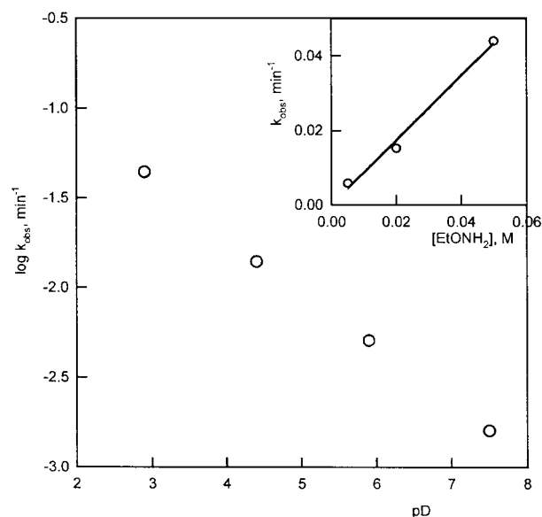
Figure 1. pD dependence of the observed pseudo-first-order rate constants for the reaction of 1 (5 mM) with O -ethylhydroxylamine (50 mM) at 60 °C in 25% \text{CD}_3\text{OD} in \text{D}_2\text{O} . Inset: plot of the pseudo-first-order rate constants for the above reaction at various concentrations of ethylhydroxylamine at pD 2.9
