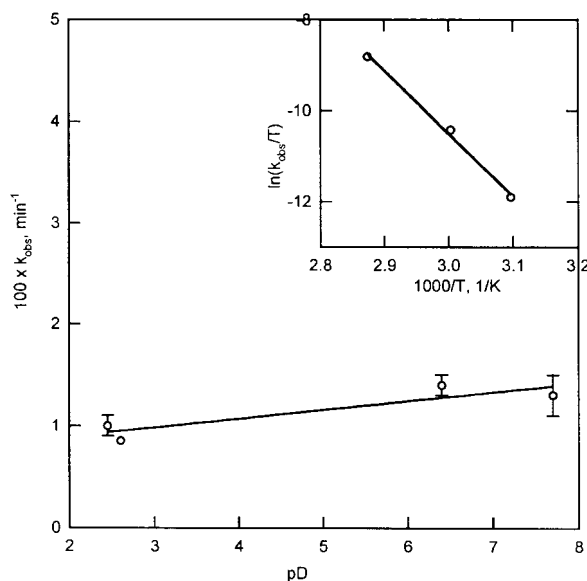
Figure 2. pH dependence of the observed pseudo-first-order rate constants for the reaction of 6 (3 mM) with O -( p -nitrophenyl)hydroxylamine (3 mM) at 60°C in D 2 O. Inset: linearized Eyring plot (see Experimental) for the above reaction at pH 3.0
